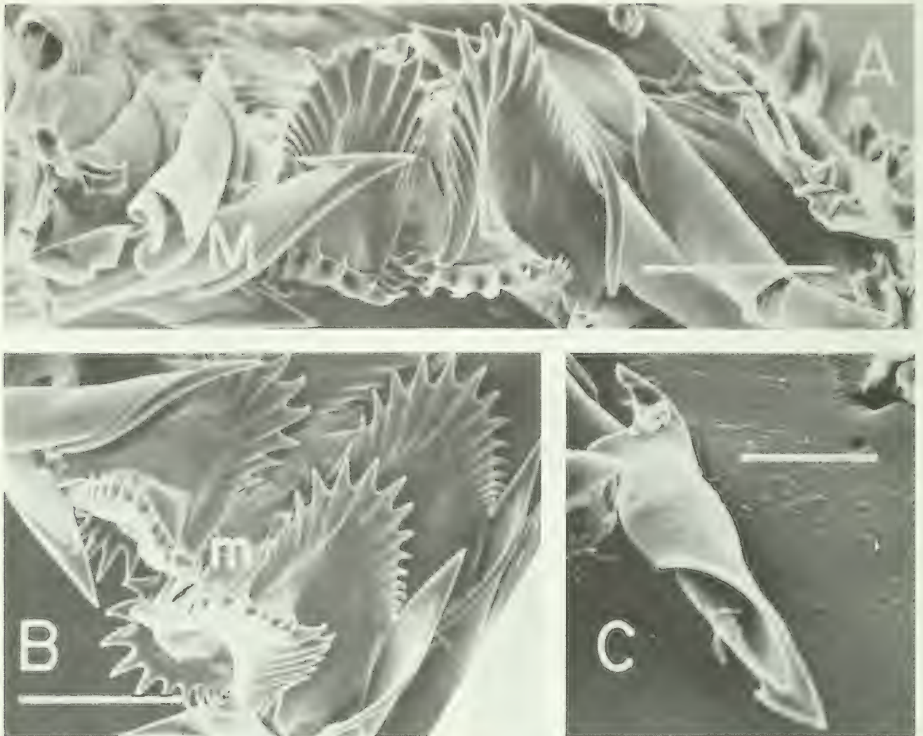
FIG. 7. Imaclava unimaculata (Sowerby, 1834) subfamily Clavinae: slicing-stabbing radula. A. Anterior view of broken radular ribbon. L = lateral tooth. M = marginal tooth. Note coiled nature of the broken marginal teeth. Scale bar = 100 \mu\text{m} . B. Dorsal view of the bending plane of the radula. m = radular membrane. Note orientation shift of the marginal teeth as they cross the bending plane. Scale bar = 100 \mu\text{m} . C. Isolated marginal tooth, note central channel and barb. Scale bar = 50 \mu\text{m} .
