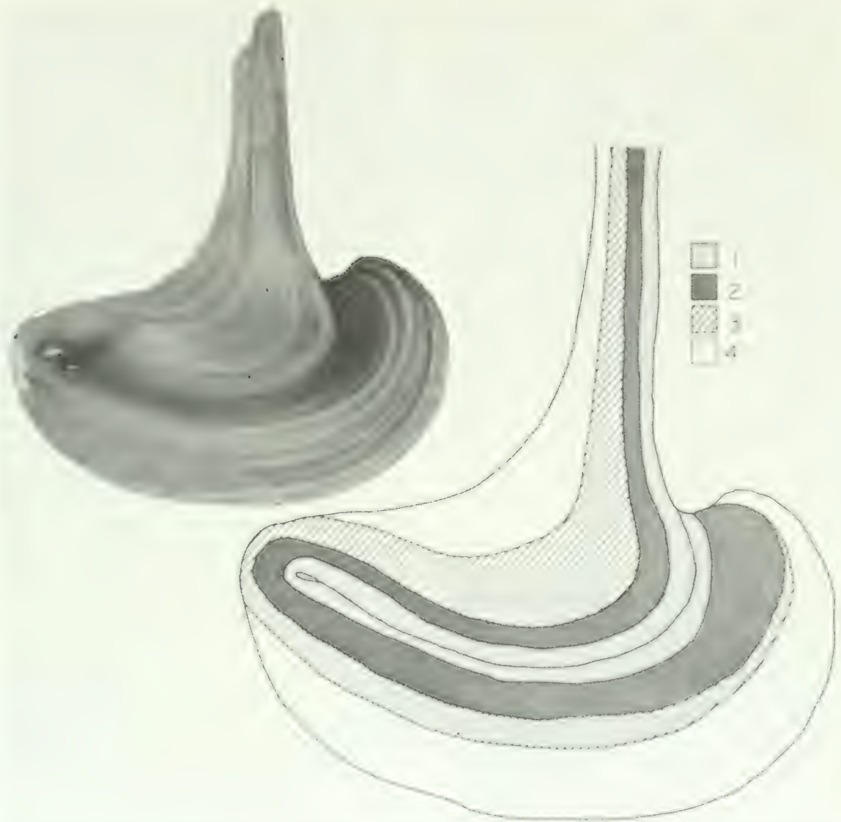
FIG. 1. Transverse thin section and schematic interpretation through the outer lip of Cassis tuberosa (Linne), showing reflection of the shell layers to form a double thickness of shell.
