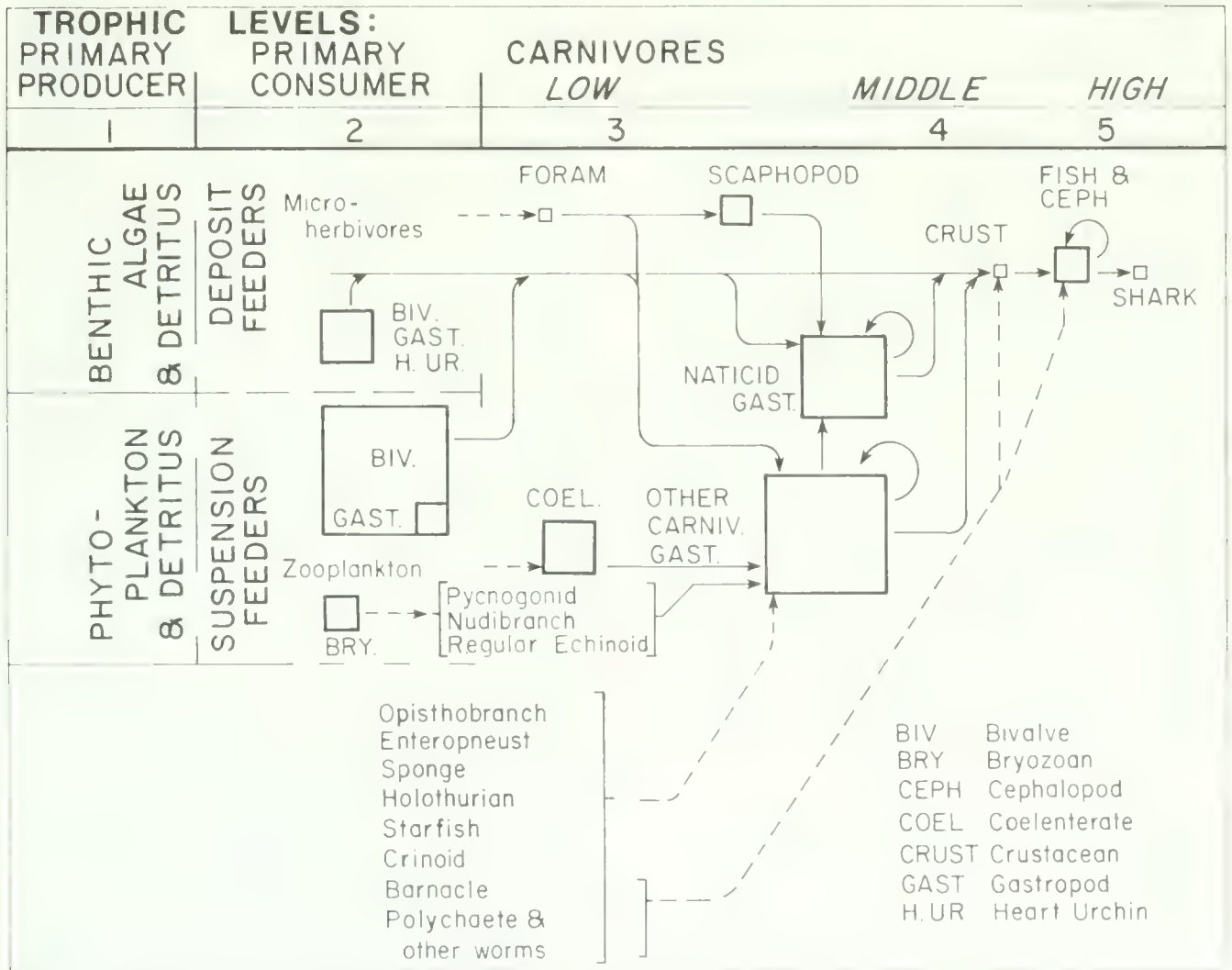
FIG. 12. Trophic web of the Main Glauconite bed community. Box sizes are proportional to numbers of individuals at each position. Solid lines and capital lettering indicate components present in the fossil assemblage and feeding relationships documented in the fossil assemblage or based on modern relationships. Dashed lines and lower case lettering indicate inferred components and relationships in the original assemblage based on modern trophic data involving components not preserved.
